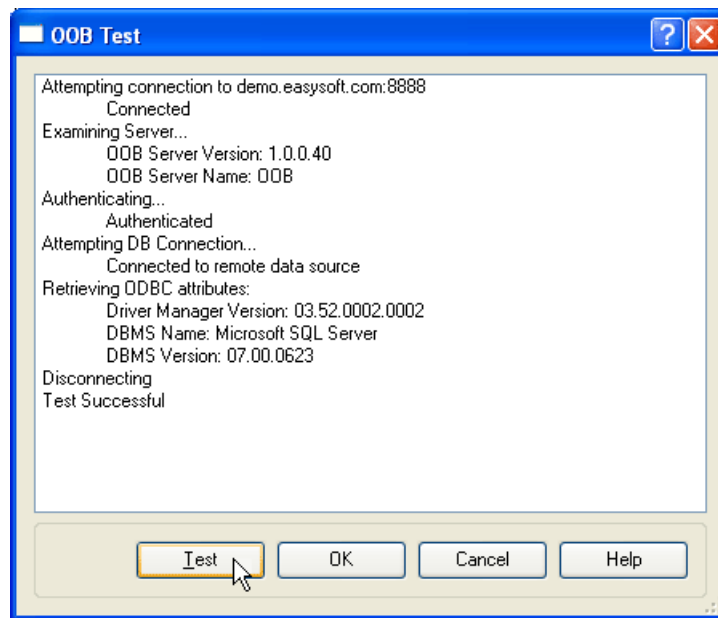
Figure 45: The OOB Test dialog box showing test results generated from valid DSN settings
