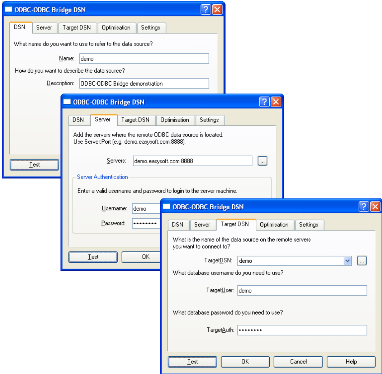
Figure 42: The DSN set up for the Easysoft demo data source
