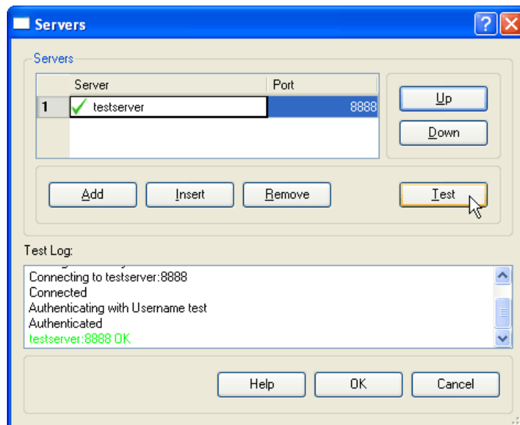
Figure 40: The Servers dialog box dialog box showing output from a successful connection to an OOB server.
