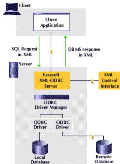
Figure 3: Easysoft XML-ODBC Server deployment
