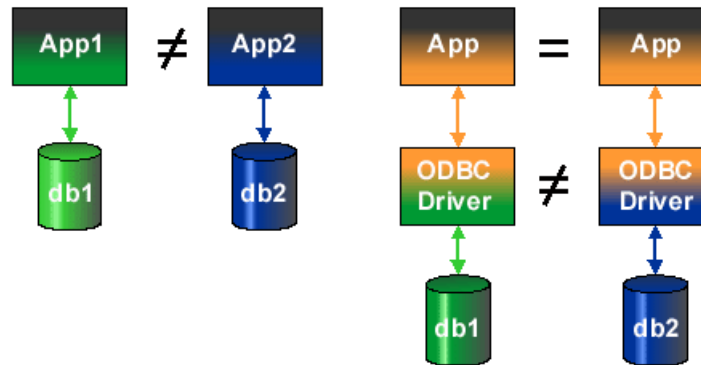
Figure 1: ODBC driver architecture
