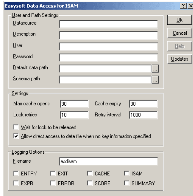
Figure 22: The Easysoft Data Access for ISAM configuration dialog box
