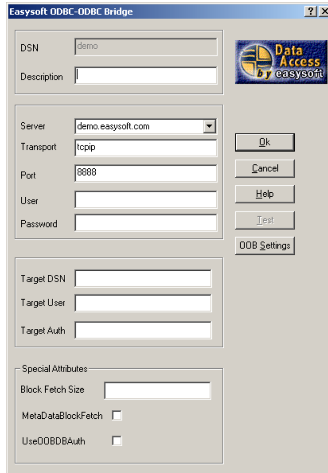
Figure 19: The Easysoft ODBC-ODBC Bridge DSN dialog box
