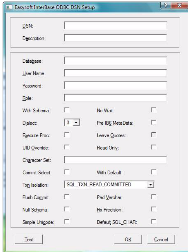
Figure 4: The Easysoft ODBC-Firebird Driver DSN Setup dialog box
